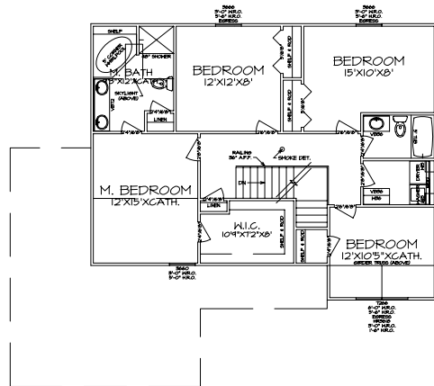
SECOND FLOOR PLAN A-5 SCALE: 1/4"=1'-0"
