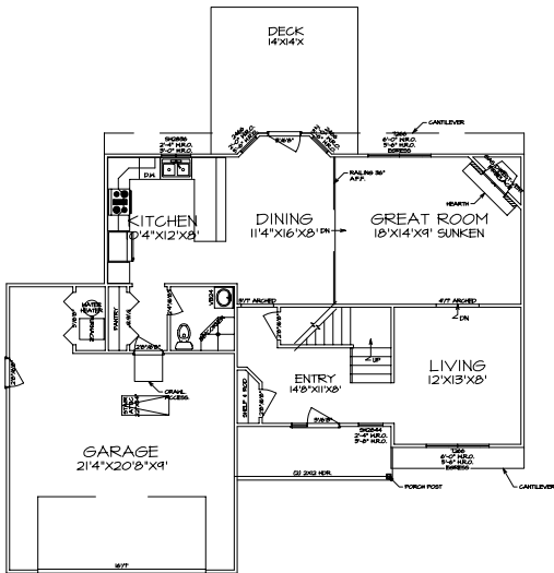
FIRST FLOOR PLAN A-4 SCALE: 1/4"=1'-0"
