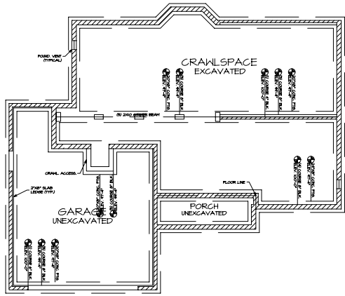
FOUNDATION PLAN A-3 SCALE: 1/4"=1'-0"
